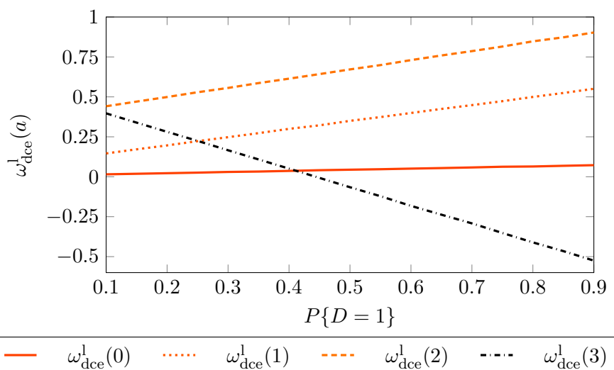
Figure 2: Weights \omega_{\text{dce}}^1(a) as a function of p when \{A|D = 1\} \sim \text{Bi}(3, 0.8) , and \{A|D = 0\} \sim \text{Bi}(3, 0.2)
