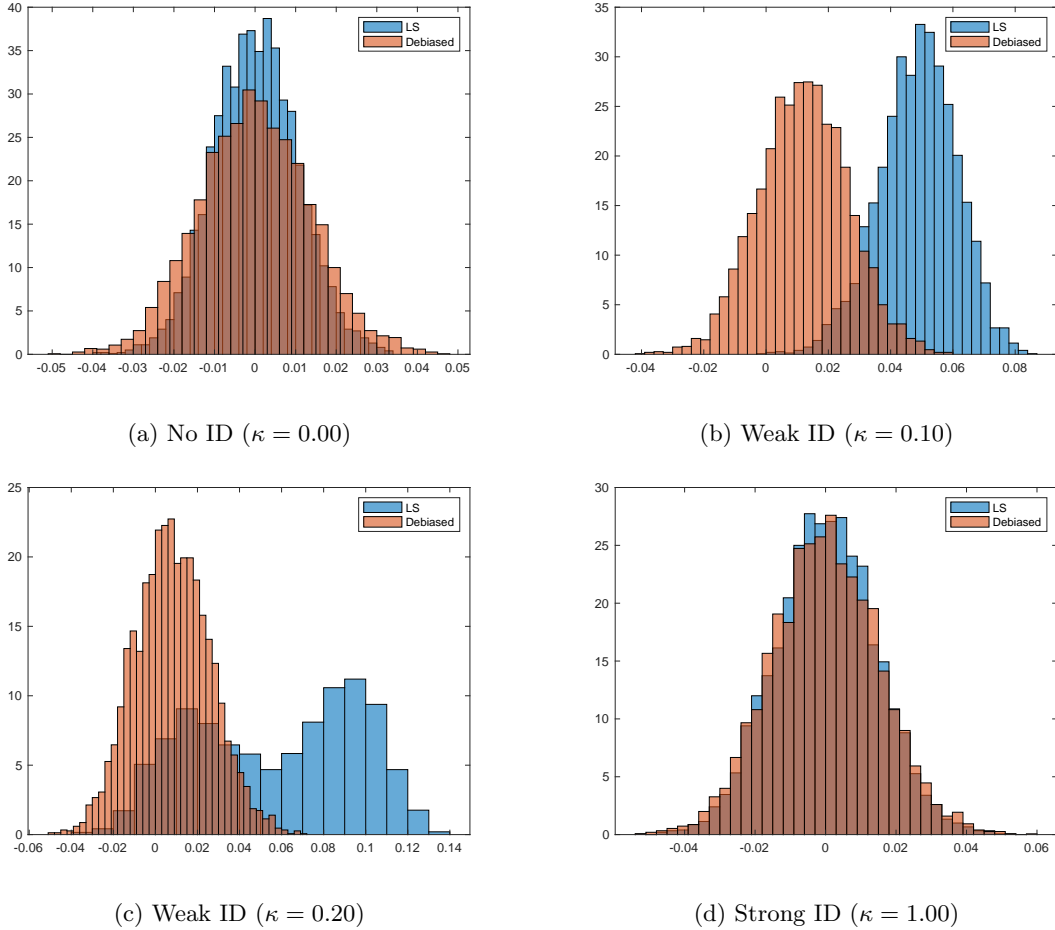
Figure 1: Finite sample distributions of the LS and the debiased estimators, N = 100 , T = 50 , R = 1
