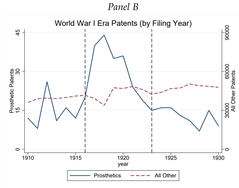
Appendix Figure D.6: Patent Time Series Note: This figure presents annual time series on patents, using USPTO categories as reported in Berkes (2018). In both panels, the solid blue line corresponds with patents from USPTO class 623 “Prosthesis.” In the top panel, the patents are organized in accordance with the year in which the patent was issued, while in the bottom panel, the patents are organized in accordance with the year in which the patent was filed.
