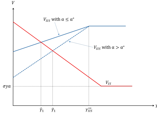
Figure 2: V_{IIS} and V_{IS} with respect to \gamma when \bar{y} \leq k
