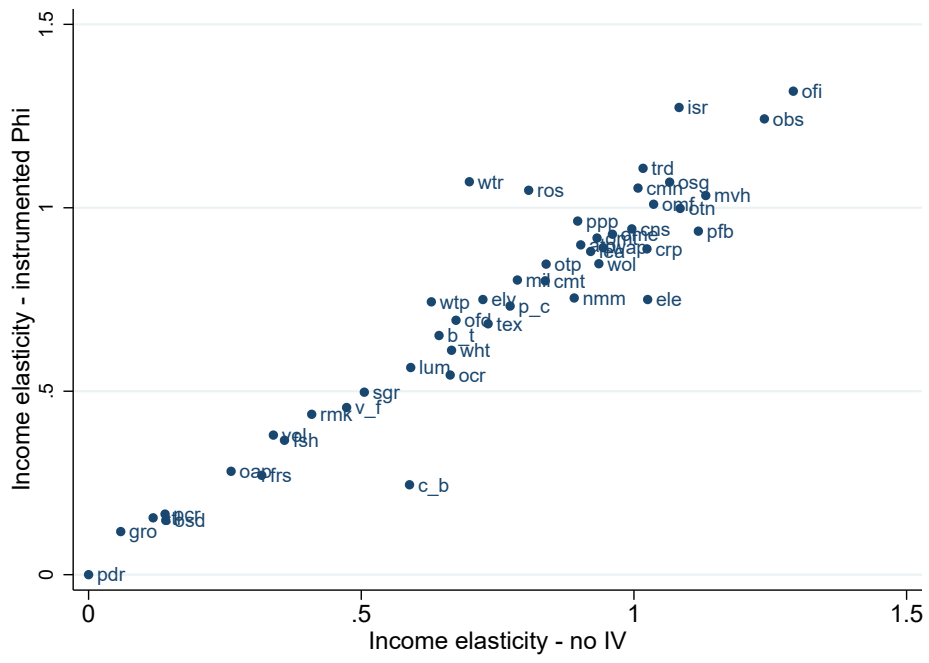
Figure A.2: Estimated income elasticities – Instrumenting \Phi
