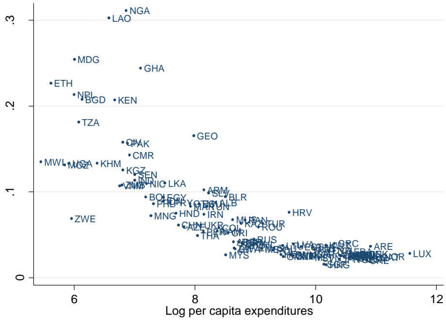
Figure 3: Simulated elasticity of the skill premium to TFP
